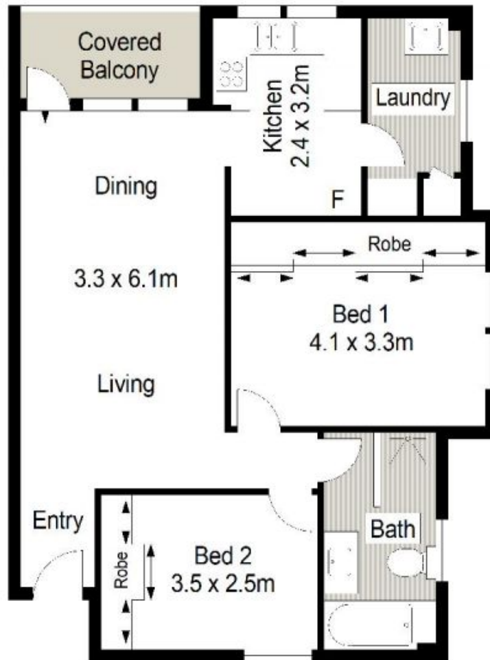
SECOND FLOOR
