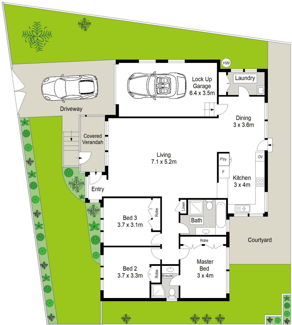
GROUND FLOOR
