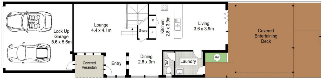
GROUND FLOOR
