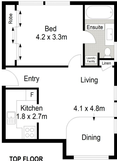
TOP FLOOR
