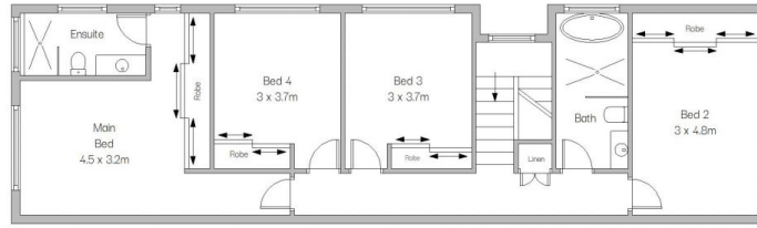
FIRST FLOOR
