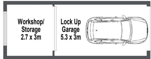
BASEMENT
